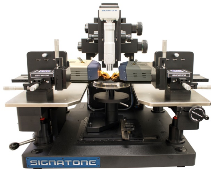
Configured with S-LAP90's and Frequency Extenders
