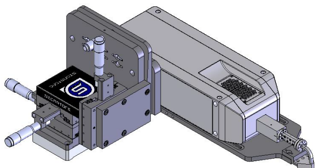
Rohde & Schwarz Frequency Extender Mounted on S-LAP90 Positioner
